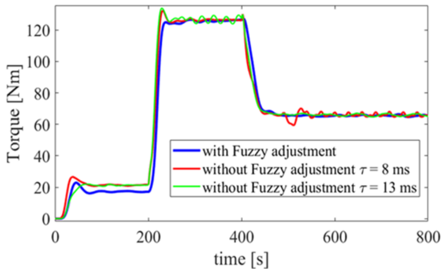
Torque regulation results using a fuzzy adaptive switching time.
