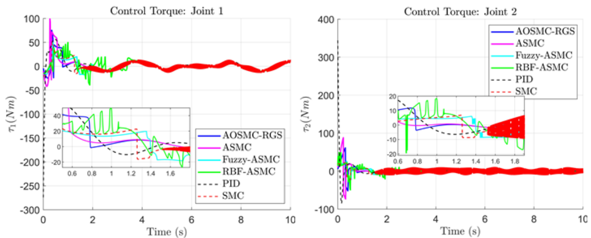
Control laws of 2-DOF robot manipulator
