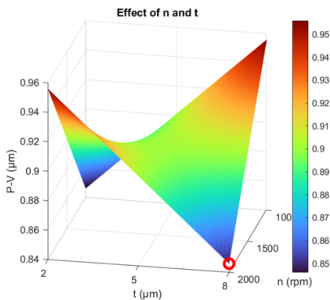
The effect of cut deep-t and spindle speed-n on form error
