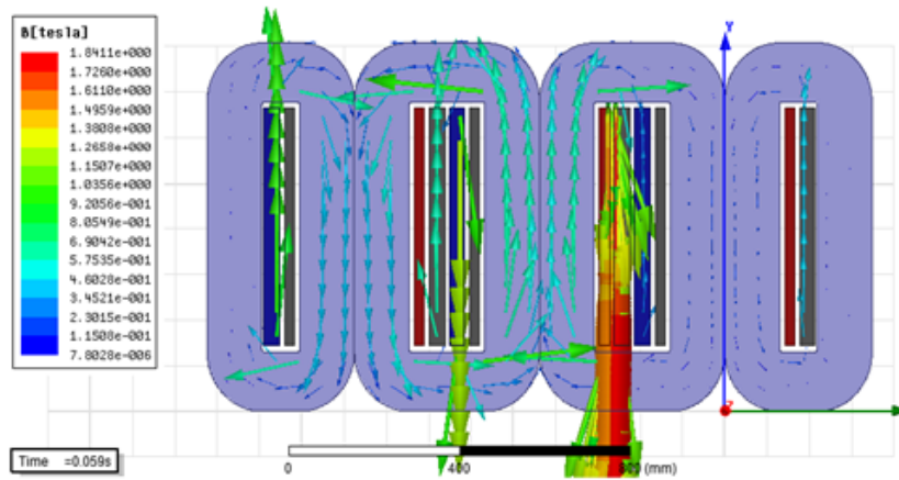
Magnetic field distribution at max short circuit current.
