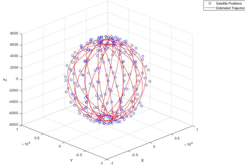
Satellite Trajectory using Non linear Least Squares and Kalman Filter
