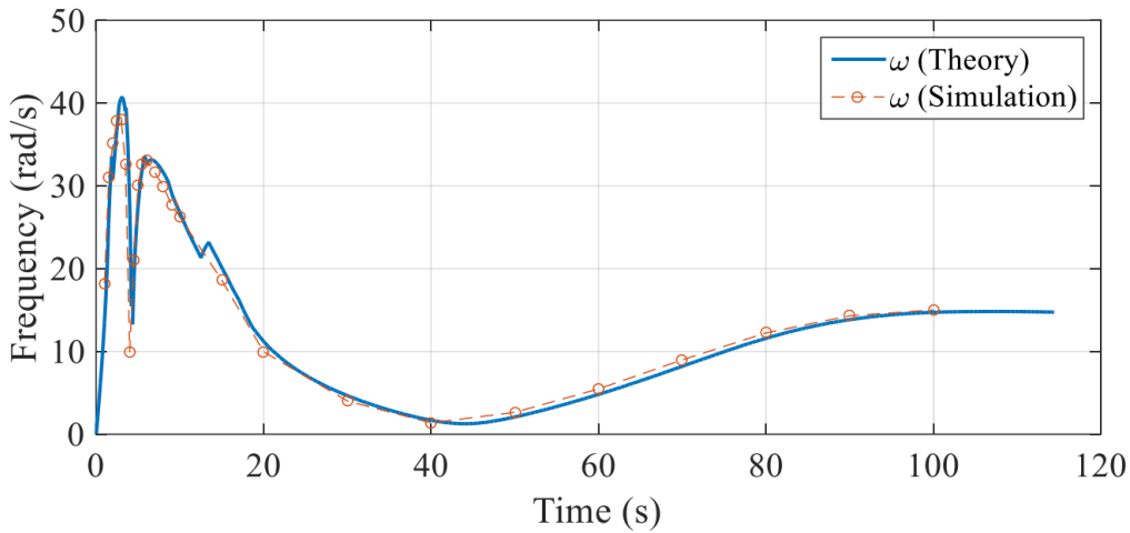
The pitching frequencies of the sounding rocket during flight obtained by different models.
