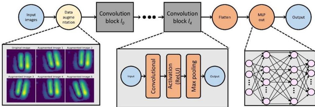
Data flow of the network and the architecture of CNN model.
