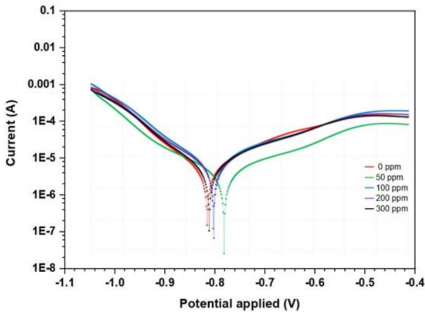
Tafel diagrams of CT3 steel at different concentrations of 1-hexadecyl-2,3-dimethylimidazolium bromide.
