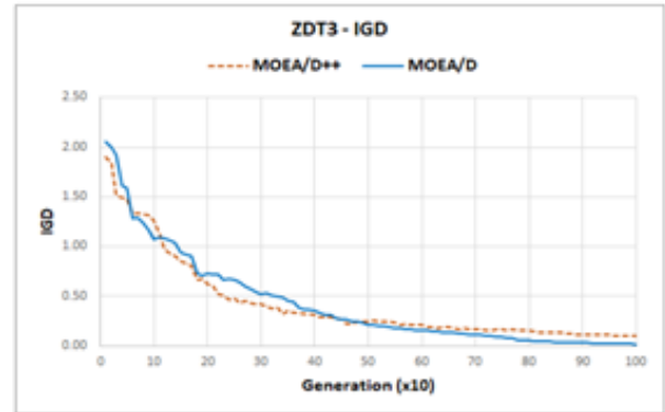
Comparison of generational distance and inverse generational distance values on ZDT3.
