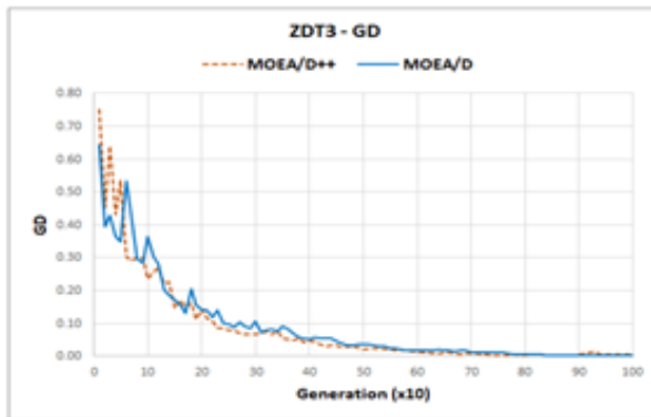
Comparison of generational distance and inverse generational distance values on ZDT3.
