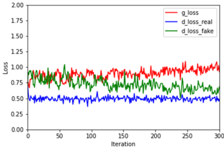
Discriminator loss with real and fake samples and Generator loss when training with malign URL strings.
