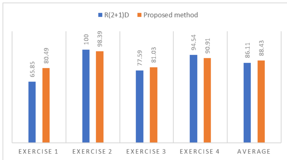
Recognition accuracy of four exercises using the proposed method versus R(2+1)D network.
