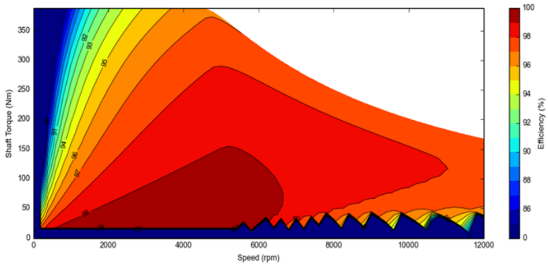
Efficiency map of hairpin winding design.
