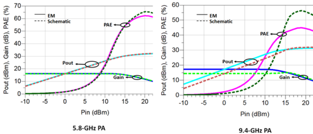
Large-signal characteristic of the designed single power amplifiers.
