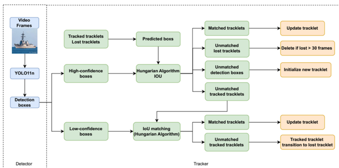
Flowchart of ship tracking using improved YOLO11n and ByteTrack.
